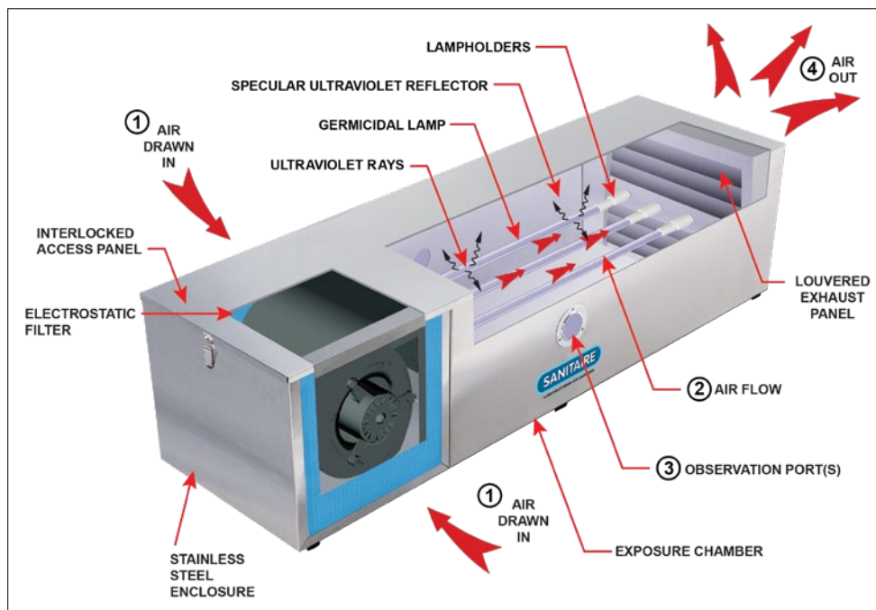
Figure 1 – SANITAIRE ® Germicidal UV Room Air Sanitizer Operation (RS435 Shown)
