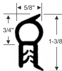
FOR 1/16" EDGES
