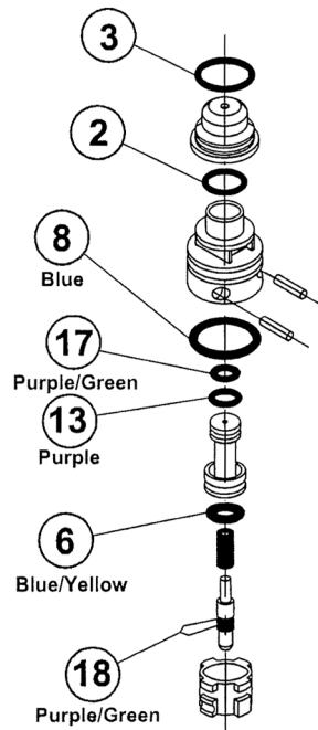
Trigger Valve Exploded View
