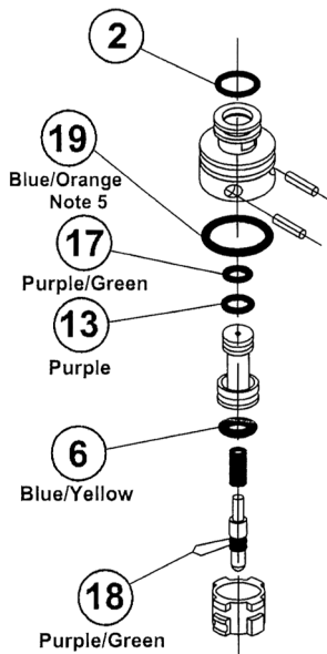
Trigger Valve Exploded View
