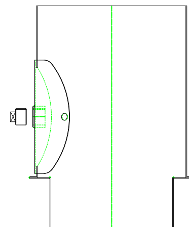
086006V0002 150mm Removable Starter Increasing Adaptor 473.0mm circ x 182.0 - 316 0.9mm R23A 390.0mm circ x 51.0 - 316 0.9mm R23A
