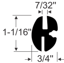
40-0496-257 • per/ft. USES 30-0439-257 LOCKSTRIP
