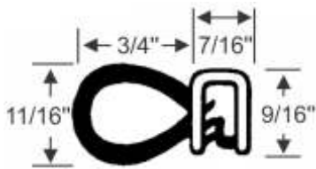
FOR 1/16" TO 1/8" EDGES 70-3582-277 • per/ft.
