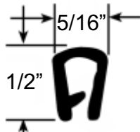
FOR 1/8" EDGES 70-3601-244 • per/ft.
