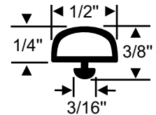
FIT IN TRACK BOTTOM OF DOOR SEALS
