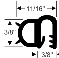
FOR 1/8" EDGES 70-3855-277 • per/ft.
