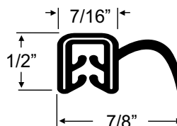
FOR 1/16" TO 1/8" EDGES 70-3801-277 • per/ft.
