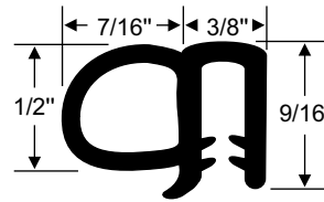
FOR 1/8" EDGES 70-3592-277 • per/ft.
