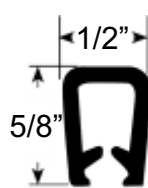
FOR 3/16" TO 1/4" EDGES 70-3598-244 • per/ft.
