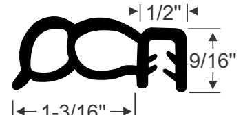
FOR 3/16" TO 1/4" EDGES 70-3885-277 • per/ft.
