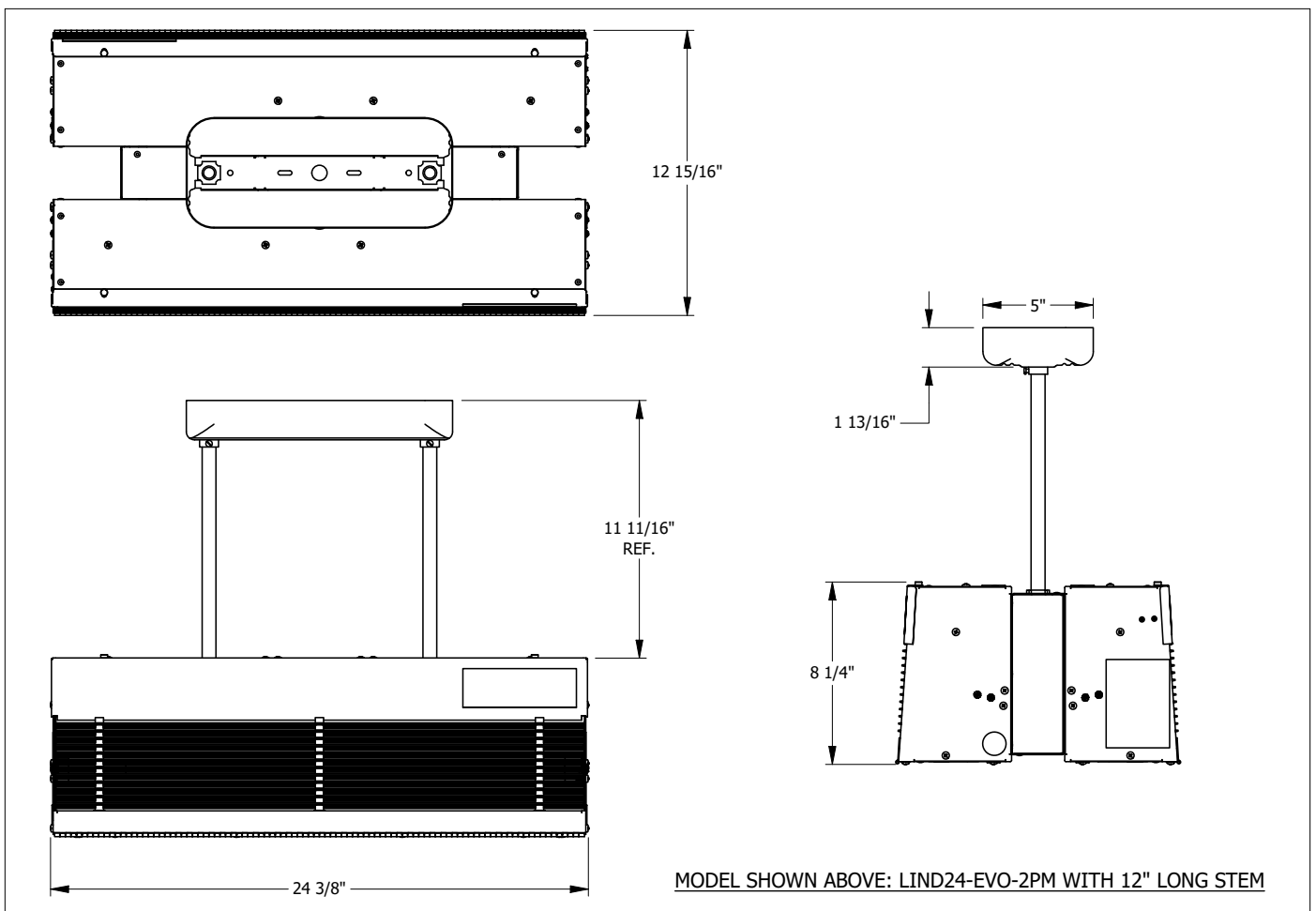
Figure 2 – LIND24-EVO-2PM Installation (Drawing Refers to “Mounting Instructions” Section)
