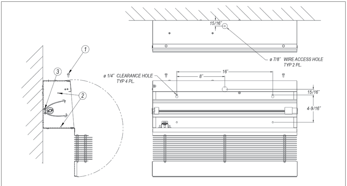
Figure 1 – LIND24-EVO & LIND24-EVO-HH Installation (Drawing Refers to “Mounting Instructions” Section)
