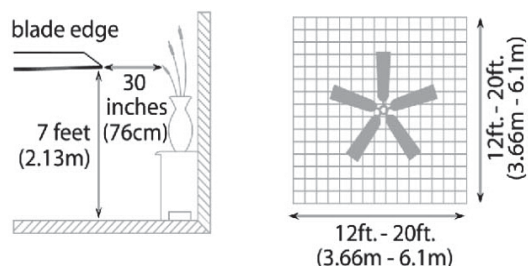
downrod installation
