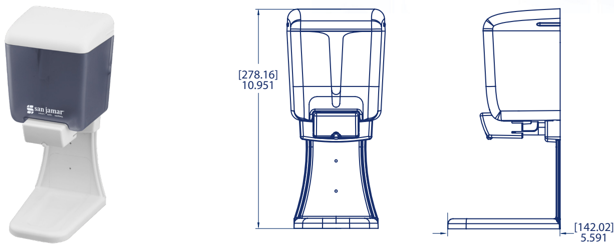
Classic soap dispenser drip tray attached to a 30 oz Classic soap dispenser
