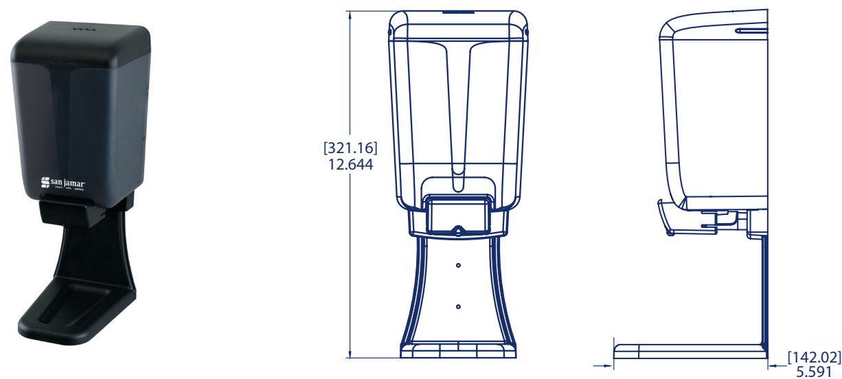
Classic soap dispenser drip tray attached to a 46 oz Classic soap dispenser
