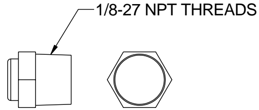
1X 5 PSI BREATHER PLUG PART NUMBER 2003PR
