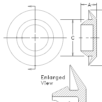
Button Plugs Flush Types
