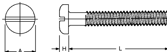
SLOTTED HEAD (NON-PREFERRED)
