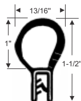
FOR 1/8" EDGES 70-3587-377 • 25 ft. Strip
