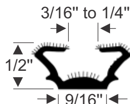
For 11/16" - 3/4" channel 70-3577-356 • 96" Strip
