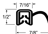
FOR 1/16" TO 1/8" EDGES 70-3801-377 • per/ft.
