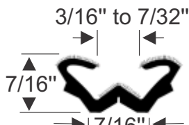
For 9/16" - 5/8" channel 70-3579-356 • 96" Strip
