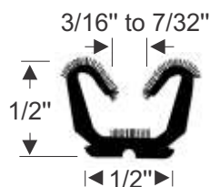
For 9/16" - 5/8" channel 70-3570-356 • 96" Strip
