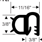
FOR 1/8" EDGES 70-3855-377 • per/ft.
