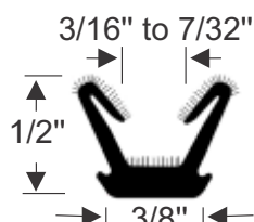
For 7/16" - 1/2" channel 70-3572-356 • 96" Strip
