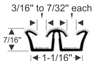
For 7/16" Individual channels Or 15/16" channels w/o divider 70-3571-356 • 96" Strip
