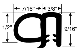
FOR 1/8" EDGES 70-3592-377 • per/ft.
