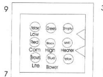
DC Harness
