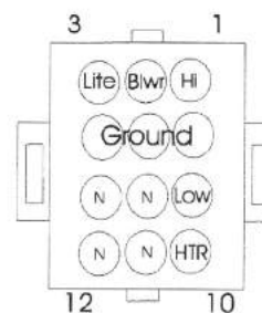
DC Harness
