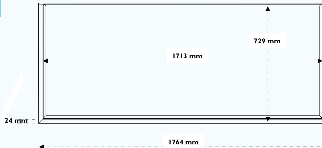
Work surface N°1 Work surface in stainless steel 304 L with built-in retention tray
