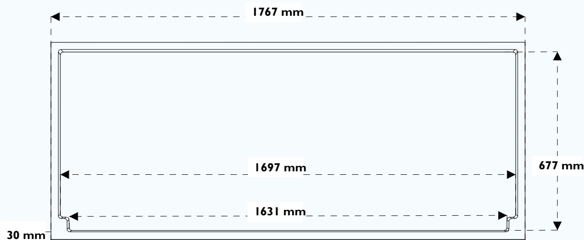
Work surface N°2 In phenolic resin with built-in retention tray
